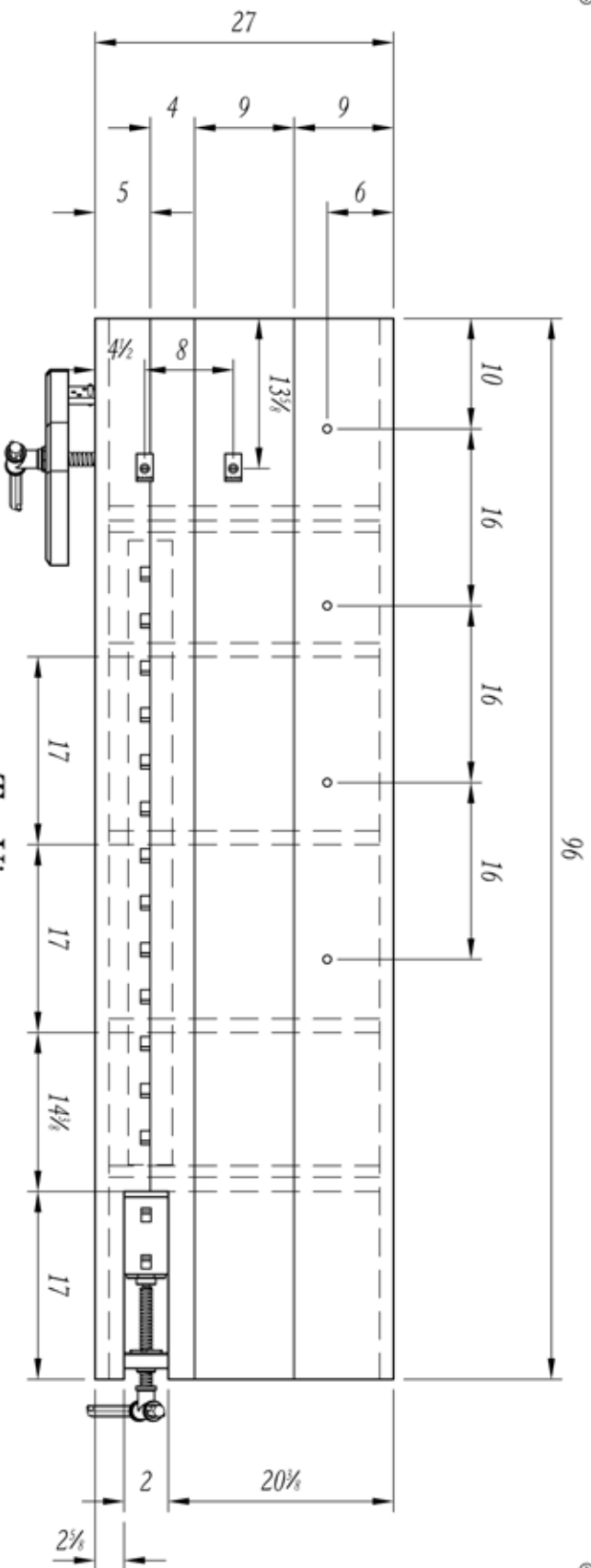
Top View
